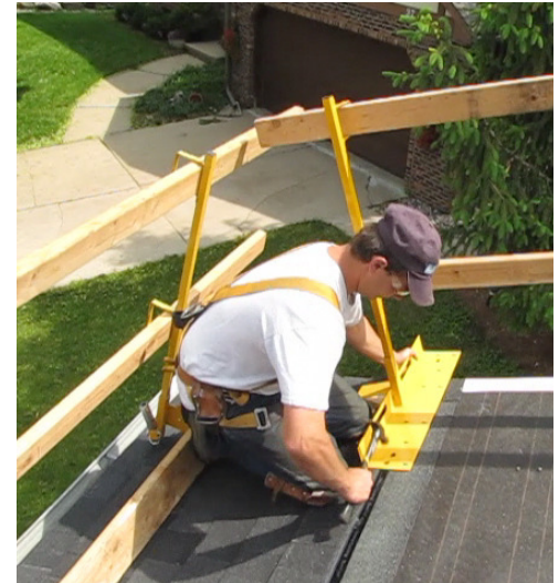
5) Secure Positioning Nail
